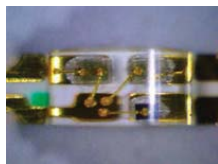
Soldering check
